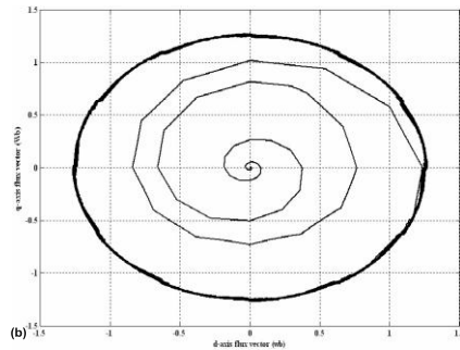
Figure 7b. Stator flux trajectory with dither injection.
