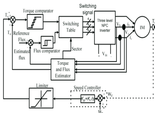
Figure 1. Block diagram of three-level inverter-fed DTC induction motor drive.
