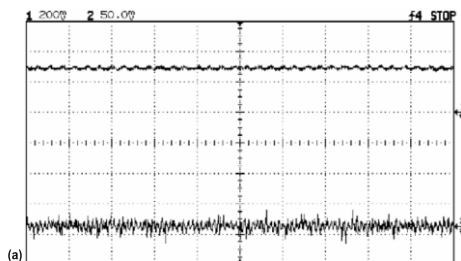
Figure 10a. Speed and electromagnetic torque when dither is not applied. Ref: 1: Speed: 500rpm/div; Ref: 2: Electromagnetic torque: 0.5N-m/div.
