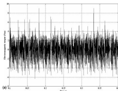
Figure 8a. Electromagnetic torque without dither injection.
