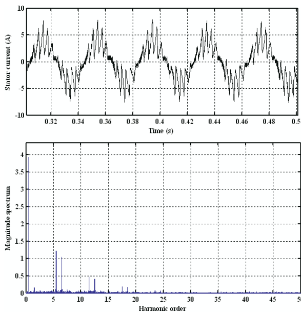
Figure 6a. Steady state stator current and harmonic spectrum without dither injection.
