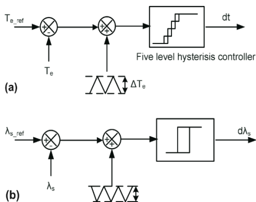
Figure 5. (a) Injection of triangular dither in torque control loop:
