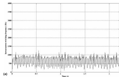
Figure 9a. Instantaneous switching frequency without dither signal.
