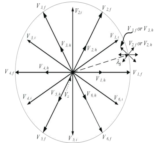
Fig.2. Output voltage vector of three-level VSI.
