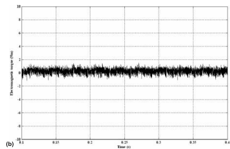
Figure 8b. Electromagnetic torque with dither injection.
