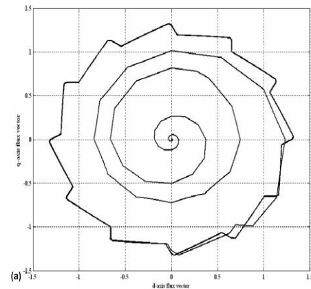
Figure 7a. Stator flux trajectory without dither injection.
