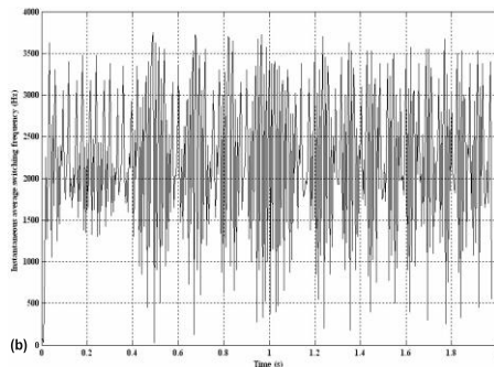
Figure 9b. Instantaneous switching frequency with triangular dither signal of 30kHz.
