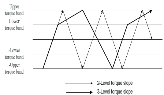
Fig.3. Torque slope pattern of three – level inverter
