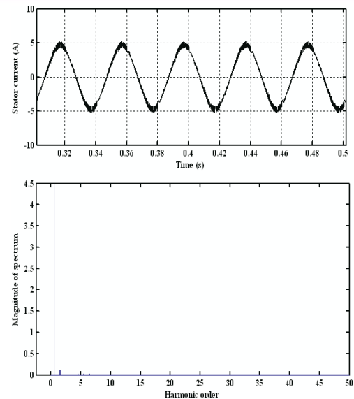
Figure 6b. Steady state stator current and harmonic spectrum with dither injection.
