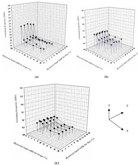
Figure4. Analytical results of convention alDTC.z-axis: Switching frequency in kHz.x-axis: Torque hysteresis band in %. y-axis: Flux hysteresis band in %. (a) No delay in the feedback loops; (b) 10 \mu s delay in the feedback loops; (c) 20 \mu s delay in the feedback loops.
