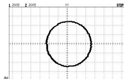
Figure 12b. Steady state stator d – q axis flux locus with triangular dither injection.
